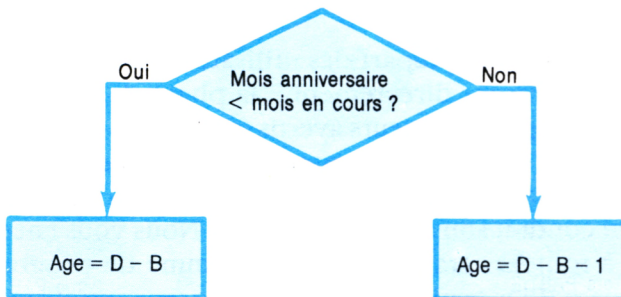
Figure 8.9 : Algorithme simple
